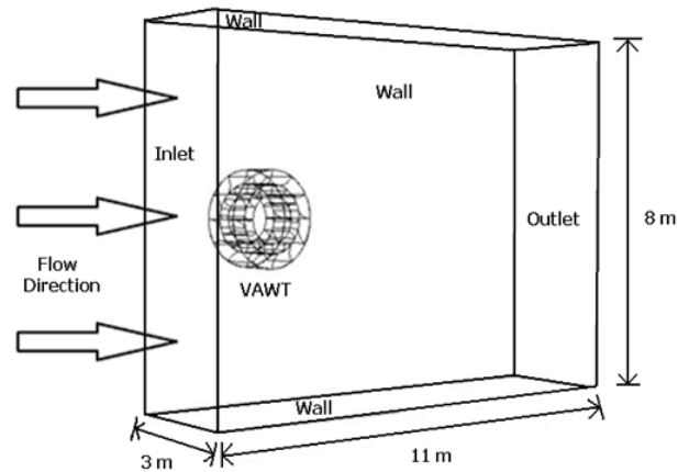
Fig. 1. Flow domain encompassing the VAWT.
