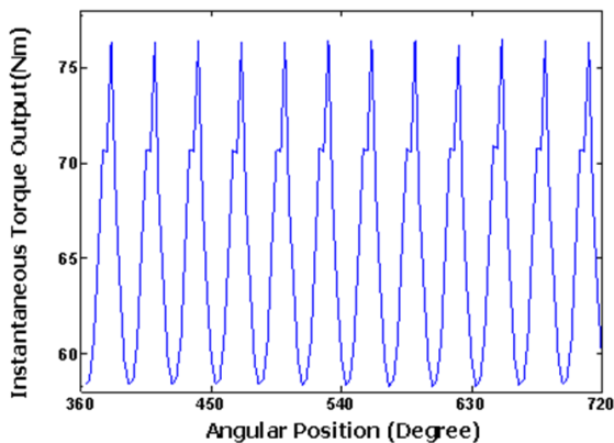
Fig. 6. Instantaneous Torque output from VAWT during steady inlet velocity of 10m/s.
