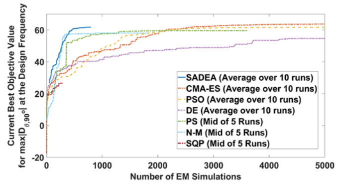
Fig. 3. Convergence graphs of all methods (Example 1).
