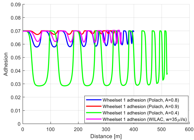
Figure 9 Wheelset1 adhesion at low adhesion condition using: Polach model with different parameter A (green, blue, red); WILAC model (magenta)
