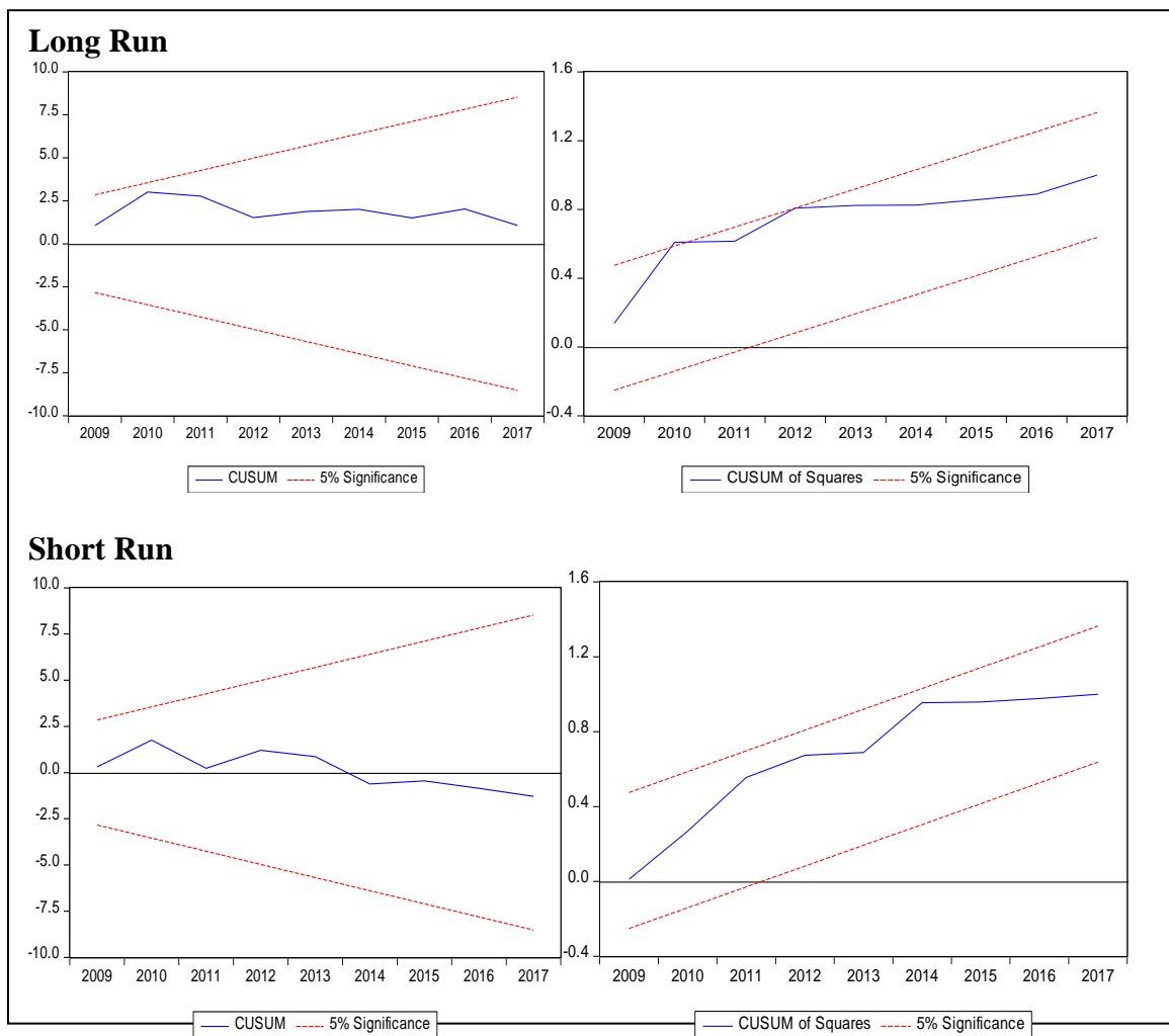
Figure-1: CUSUM and CUSUMsq
